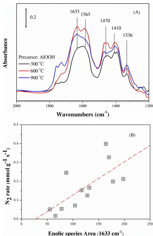
Figure 4. (A) In situ DRIFTS spectra of adsorbed species on 2 wt % Ag/Al_2O_3 catalysts derived from AlOOH (calcined at 300, 600, and 900 °C) at steady state in a flow of C_2H_5OH + O_2 at 300 °C. (B) Relationship between enolic species with N_2 production rate among different precursors.
