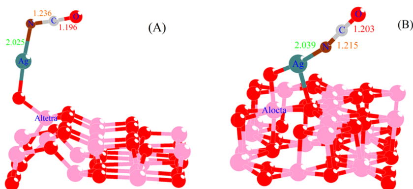
Figure 8. Structure of the \text{-NCO} adsorbed on \text{Ag/Al}_2\text{O}_3 catalyst: (A) on \text{Ag-O-Al}_{\text{tetra}} entity; (B) on \text{Ag-O-Al}_{\text{octa}} entity.
